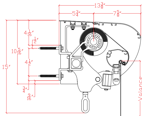
87 TRADITIONAL AWNING WITH FLEXPITCH WITH XL HOOD
