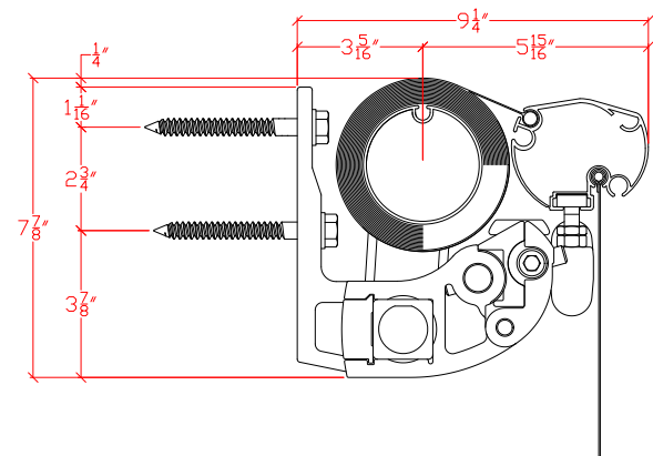
150 TRADITIONAL AWNING WITHOUT HOOD
