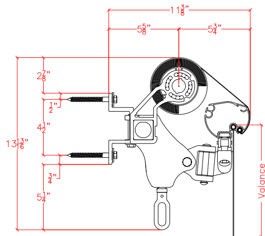
87 TRADITIONAL AWNING WITH FLEXPITCH WITHOUT HOOD
