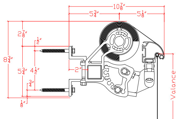
77 TRADITIONAL AWNING WITHOUT HOOD
