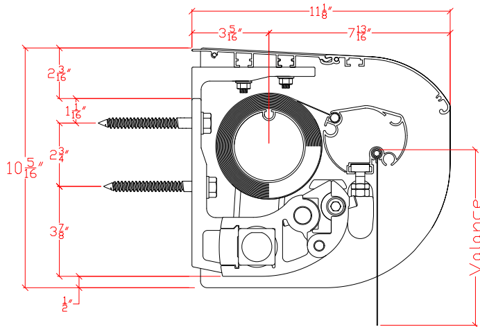
150 TRADITIONAL AWNING WITH ALUMINUM HOOD
