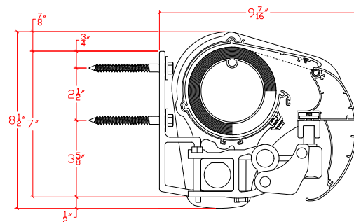
98 FULL CASSETTE AWNING
