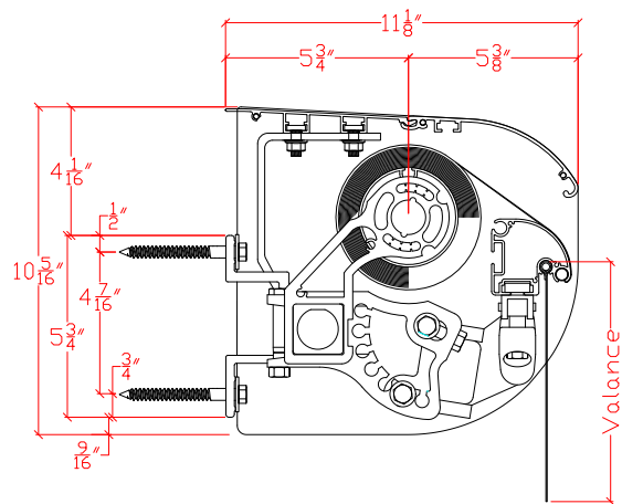
77 TRADITIONAL AWNING WITH HOOD
